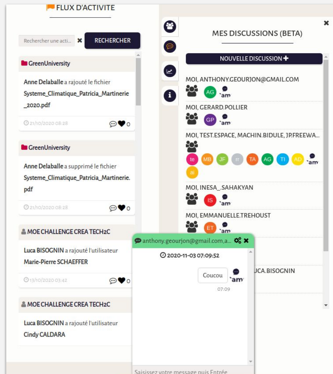
Fig2. Discussion board
