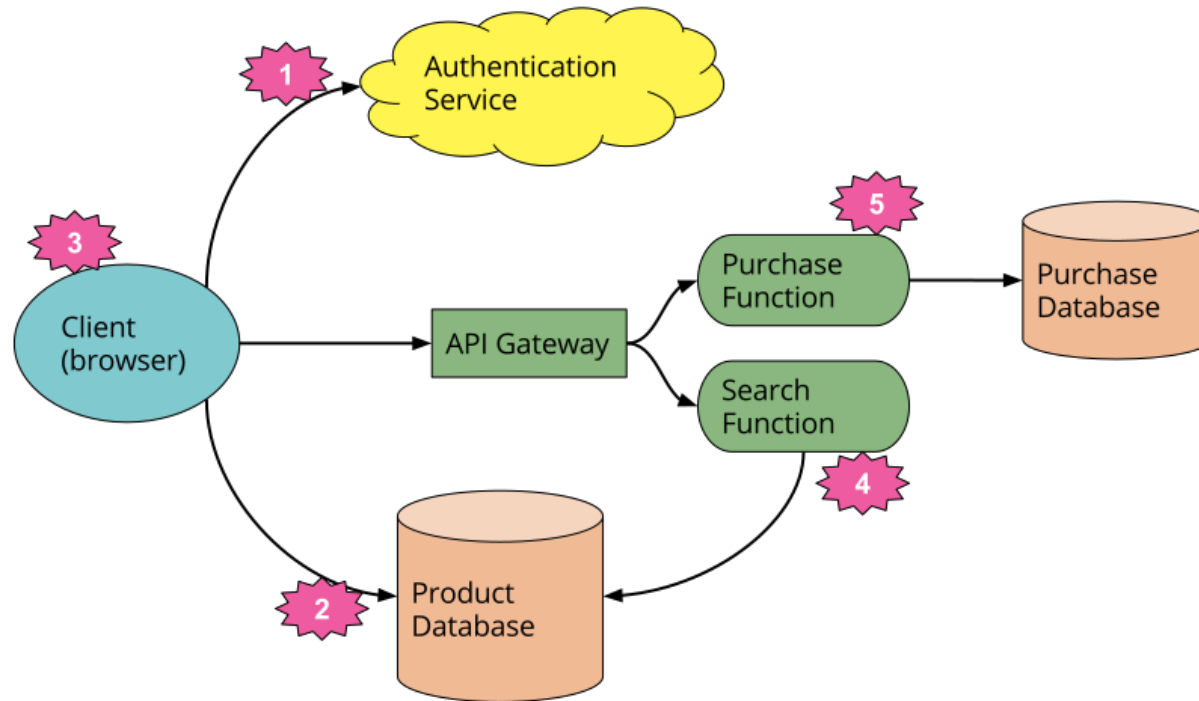
Application serverless
