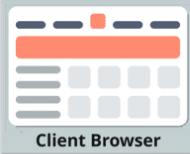
Microservice Architecture
